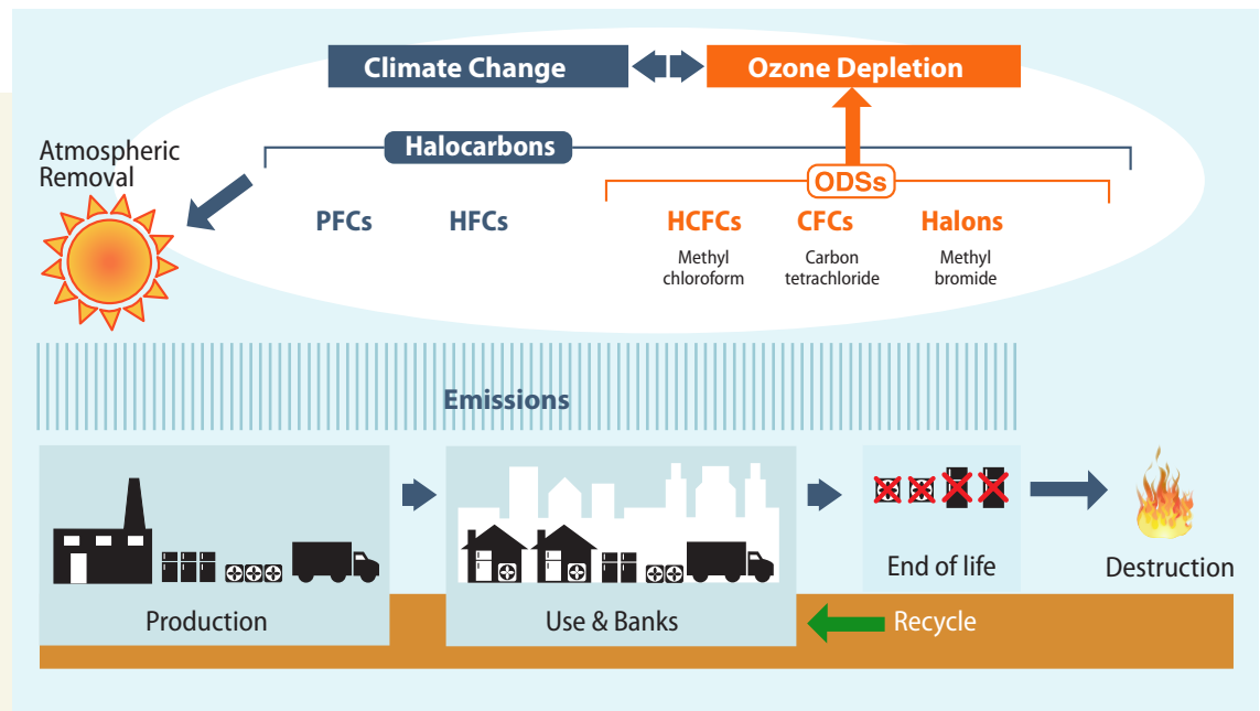
IMAGE 4: THE EFFECTS OF ODS EMISSIONS ON OZONE DEPLETION AND CLIMATE CHANGE [8]
