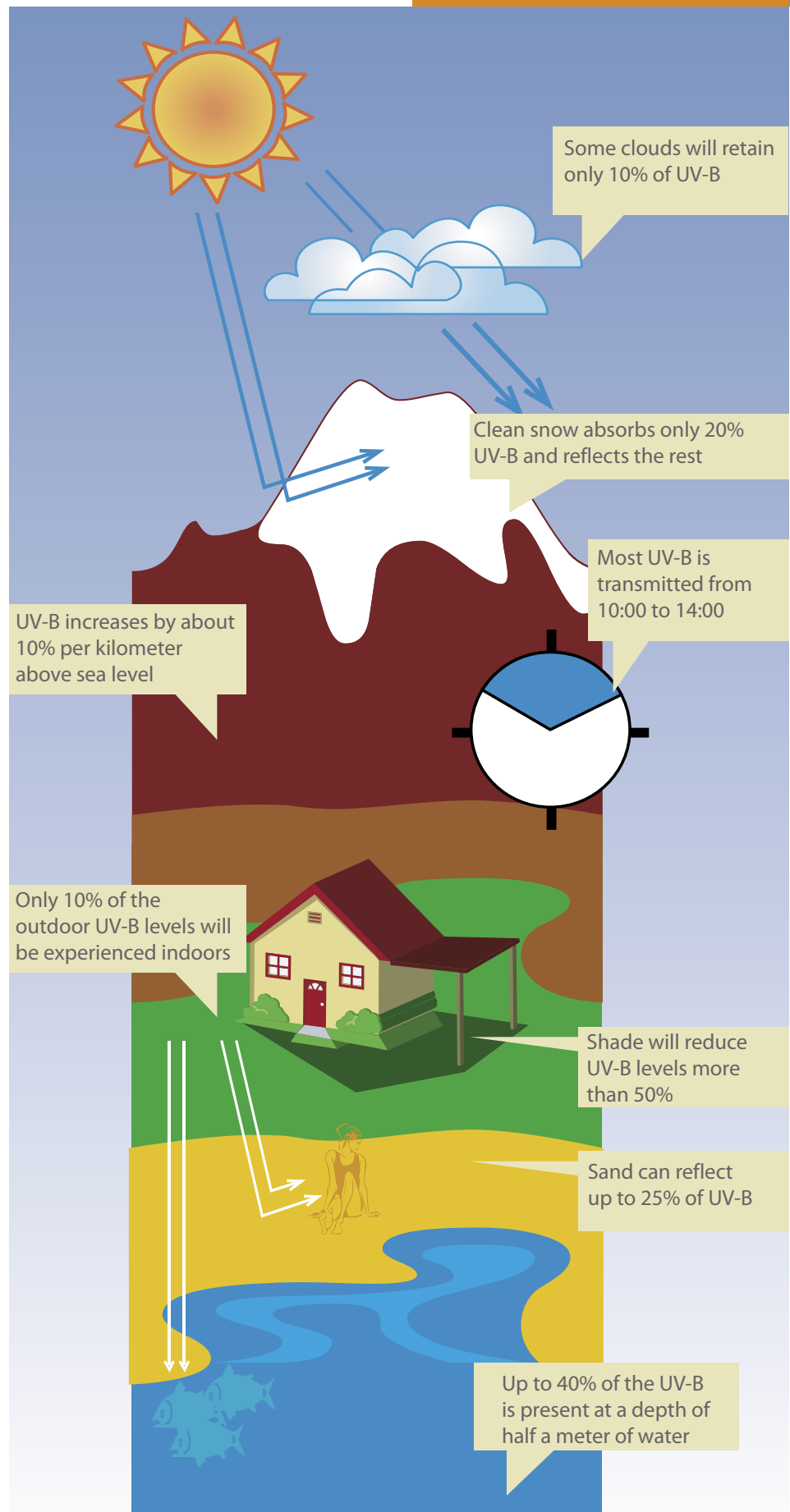
IMAGE 3: THE EFFECTS OF DIFFERENT SURFACES ON THE UV-B RECEIVED BY AN OBJECT [5]
